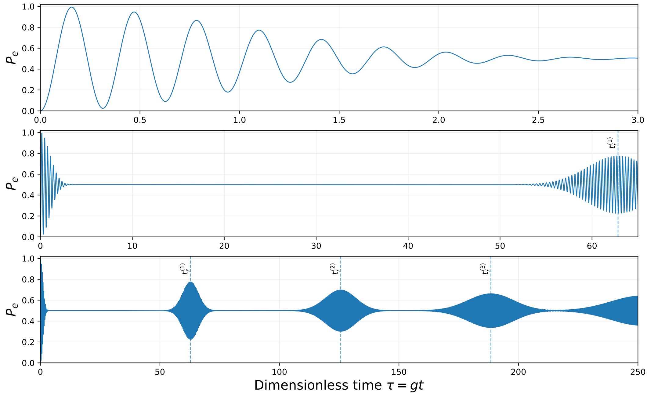
Collapse and revival for \bar{n} = 100
